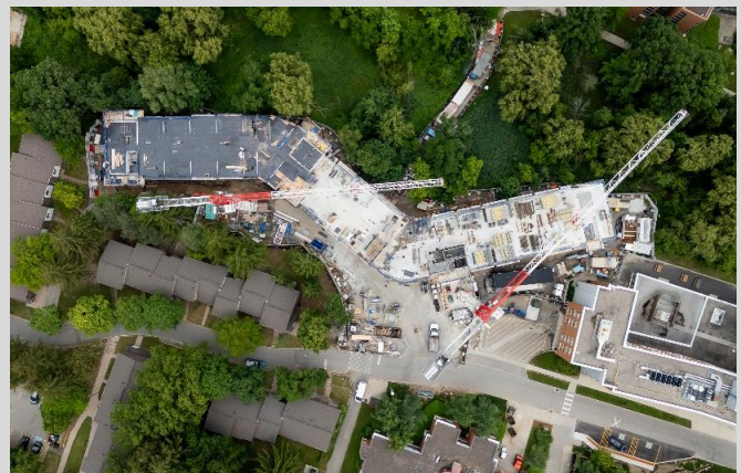
Pictured: Work on Level 5 suspended slab.
