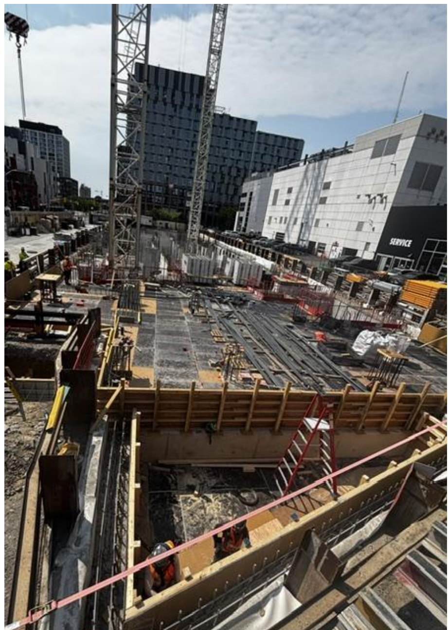
Pictured: ground floor slab deck install commenced at the north
